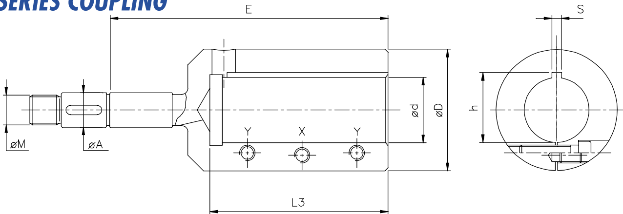
DIMENSIONAL TABLE
